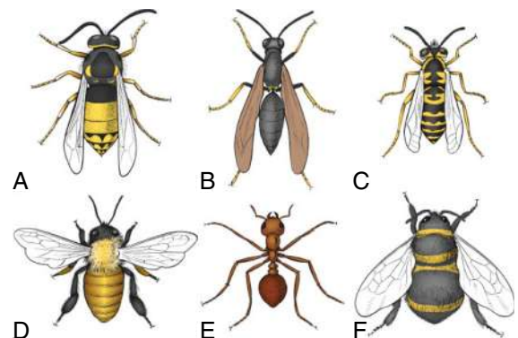
Fig. 187.1 Representative venomous Hymenoptera. A, Hornet ( Vespa maculata ). B, Wasp ( Chlorion ichneumerea ). C, Yellowjacket ( Vespa maculiforma ). D, Honeybee ( Apis mellifera ). E, Fire ant ( Solenopsis invicta ). F, Bumblebee ( Bombus species). (From Erickson TB, Marquez A. Arthropod envenomation and parasitism. In: Auerbach PS, Cushing TA, Harris NS, eds. Auerbach's Wilderness Medicine . 7th ed. Philadelphia: Elsevier; 2017: Fig 41-1, p 937.)
